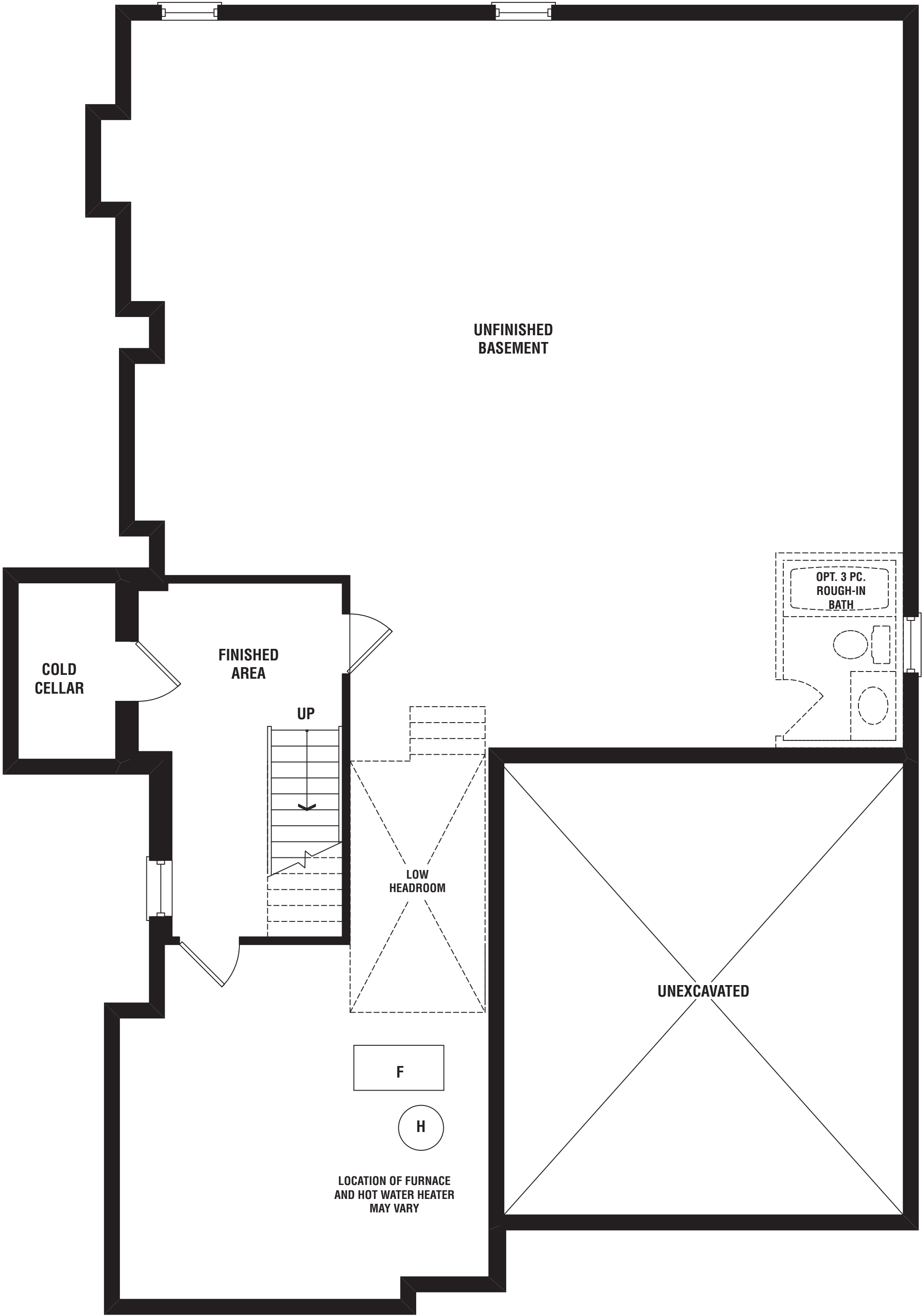
BASEMENT FLOOR ELEV. 'B'
