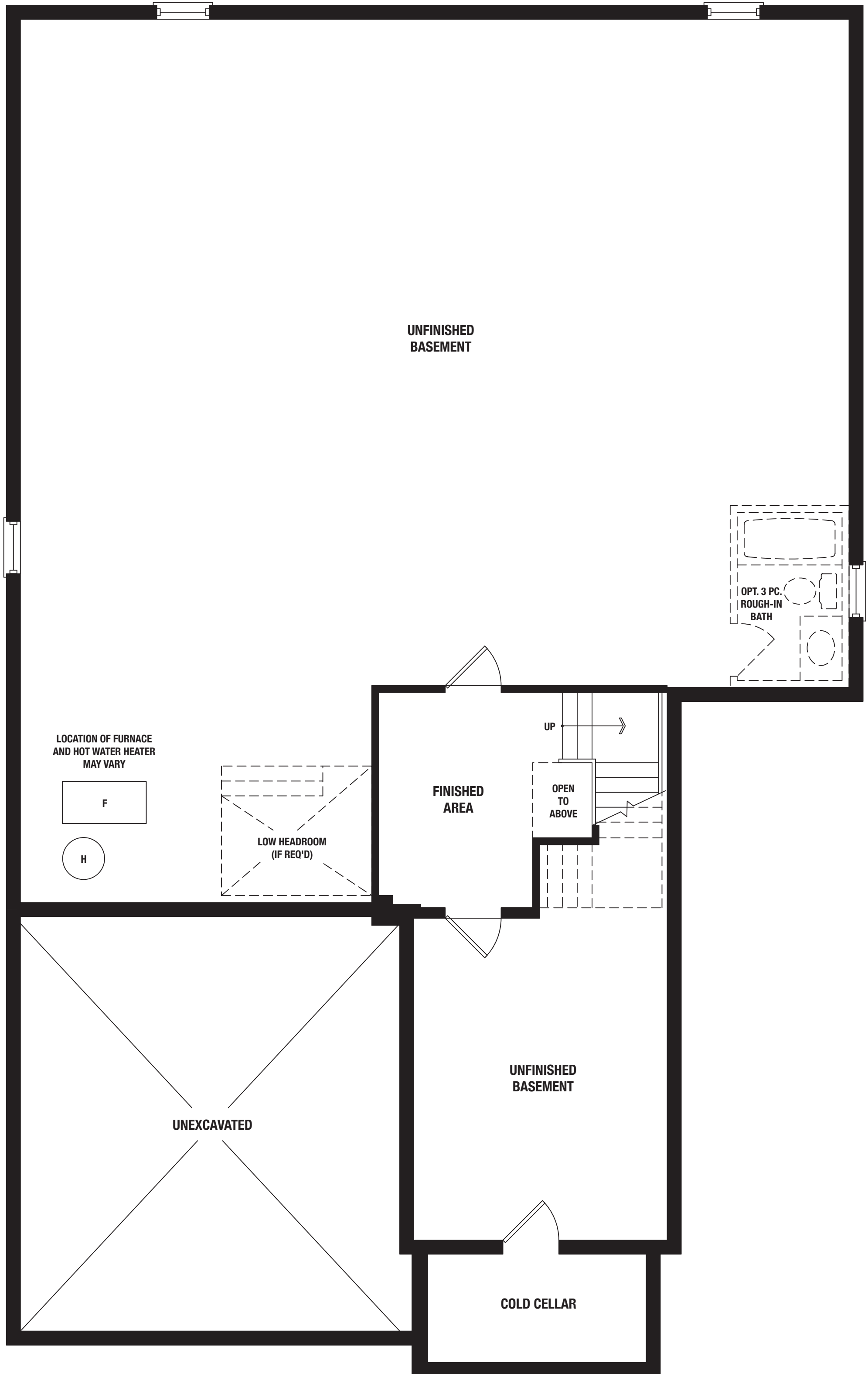
BASEMENT FLOOR ELEV. 'A' & 'B'
